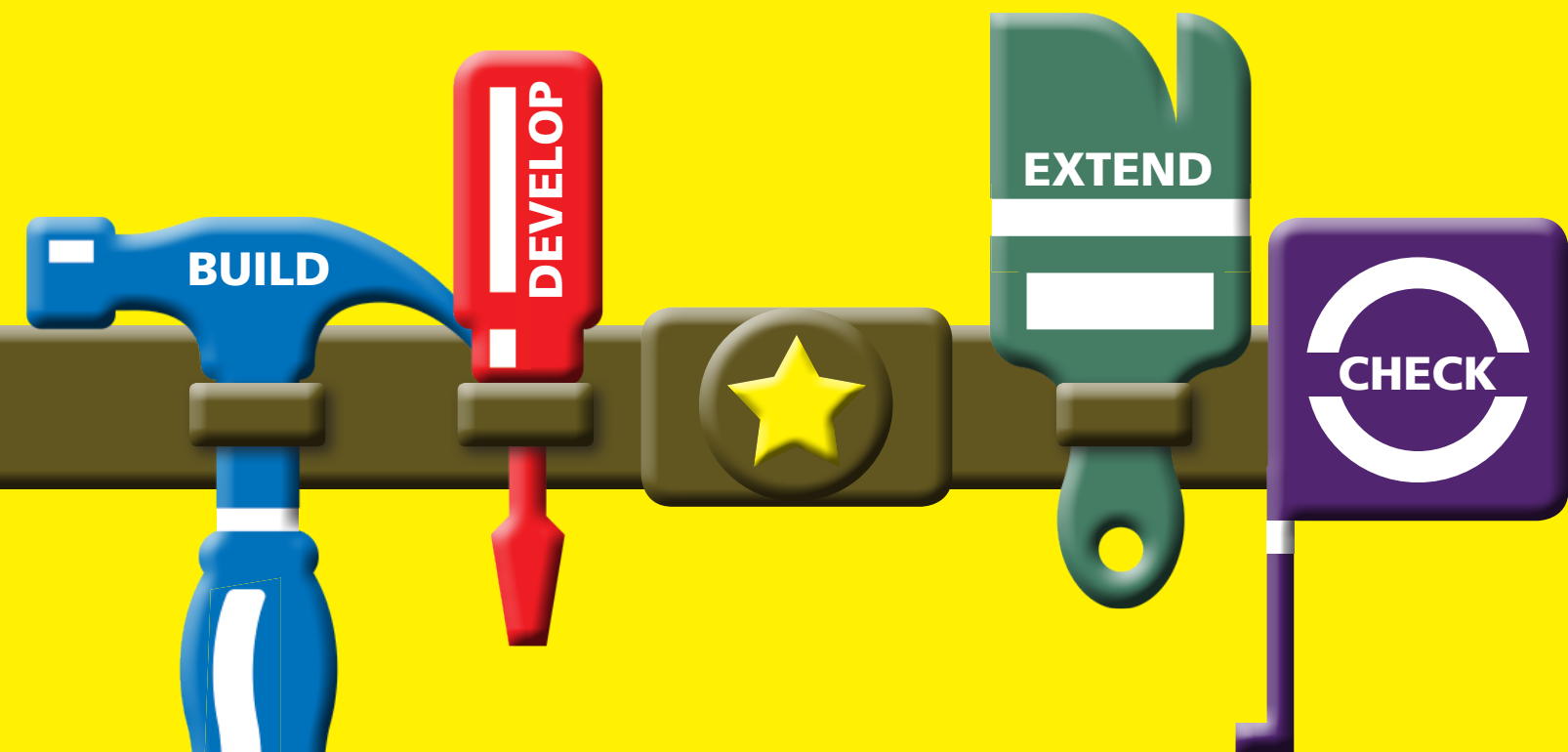
Activity Distribution for Math Programs
