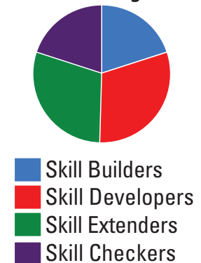
Activity Distribution for Math Programs
